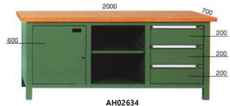
P-KW 200 Work Bench
