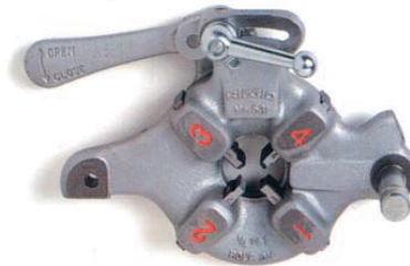
No. 531 and 532 Bolt Die Heads
