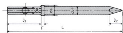
Hex Shank
